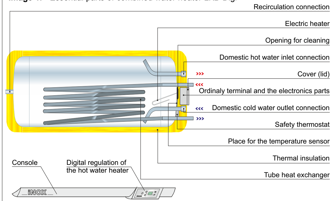
Image 1. - Essential parts of combined water heater LKB-Digi
